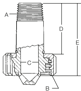
Style C For Vapor Equalizing
