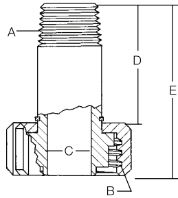
Style A For Liquid Filling
