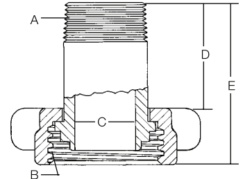
Style B For Liquid Filling
